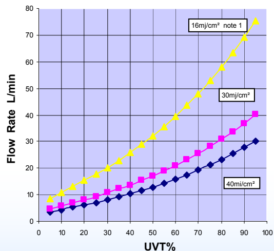
UVD320 Performance Curves note 2
